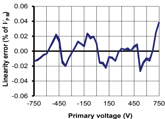
Figure 15: Typical linearity error at 25^\circ\text{C}
