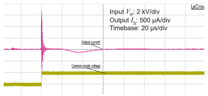
Figure 12: Detail of typical common mode perturbation (2000 V step with 6 \text{ kV}/\mu\text{s} , R_M = 100 \Omega )
