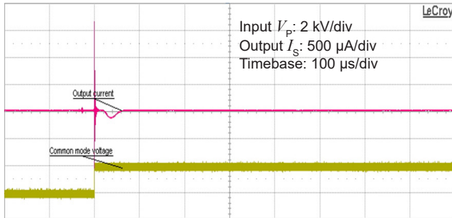
Figure 11: Typical common mode perturbation (2000 V step with 6 \text{ kV}/\mu\text{s} , R_M = 100 \Omega )
