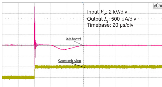
Figure 12: Detail of typical common mode perturbation (250 V step with 6 kV/μs, R_M = 100 \Omega )
