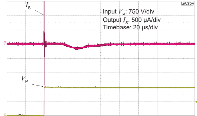
Figure 12: Detail of typical common mode perturbation (1500 V step with 6 \text{ kV}/\mu\text{s} , R_M = 100 \Omega )
