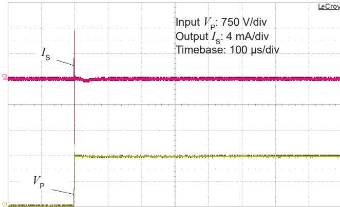
Figure 11: Typical common mode perturbation (1500 V step with 6 \text{ kV}/\mu\text{s} , R_M = 100 \Omega )
