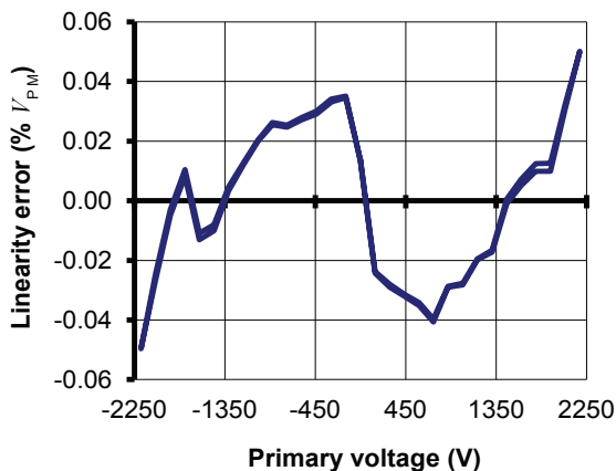
Figure 15: Typical linearity error at 25^\circ\text{C}
