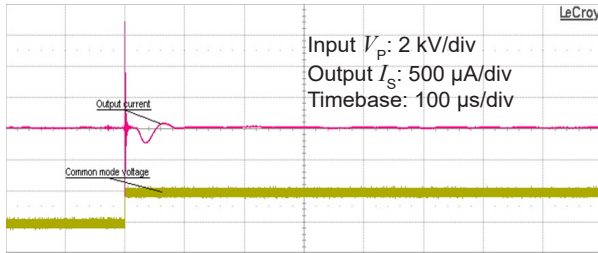
Figure 11: Typical common mode perturbation (2000 V step with 6 \text{ kV}/\mu\text{s} , R_M = 100 \Omega )
