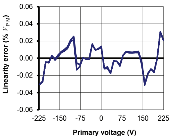
Figure 15: Typical linearity error at 25^\circ\text{C}
