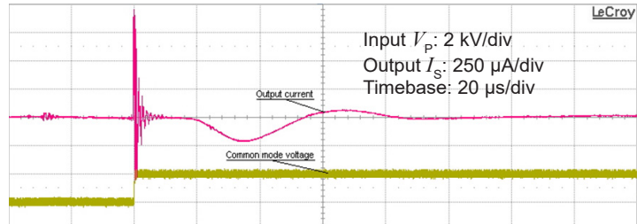
Figure 12: Detail of typical common mode perturbation (2000 V step with 6 \text{ kV}/\mu\text{s} , R_M = 100 \Omega )
