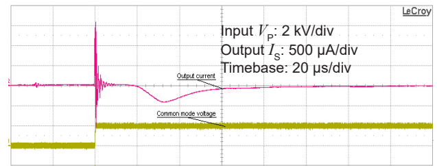
Figure 12: Detail of typical common mode perturbation (2000 V step with 6 kV/μs, R_M = 100 \Omega )
