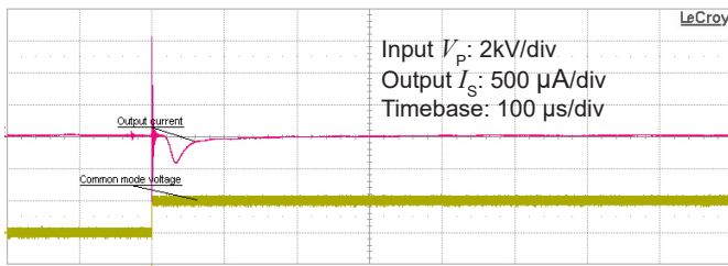
Figure 11: Typical common mode perturbation (2000 V step with 6 kV/μs R_M = 100 \Omega )
