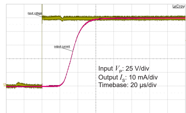
Figure 6: Typical step response (0 to 125 V)
