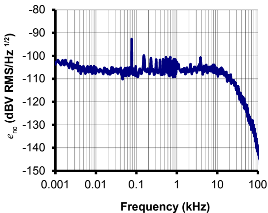
Figure 13: Typical output RMS noise voltage spectral density of e_{no} with R_M = 50 \Omega
