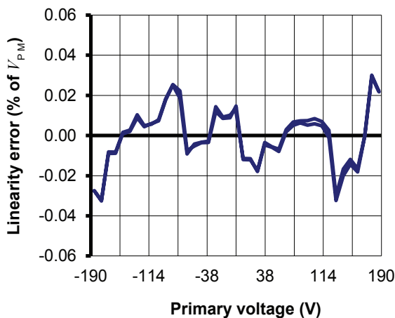
Figure 15: Typical linearity error at 25 °C
